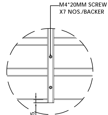
DETAIL 'C' SCALE1:4
