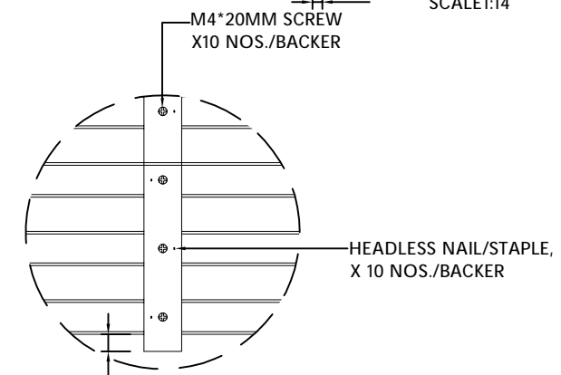
DETAIL 'C' SCALE:1:4
