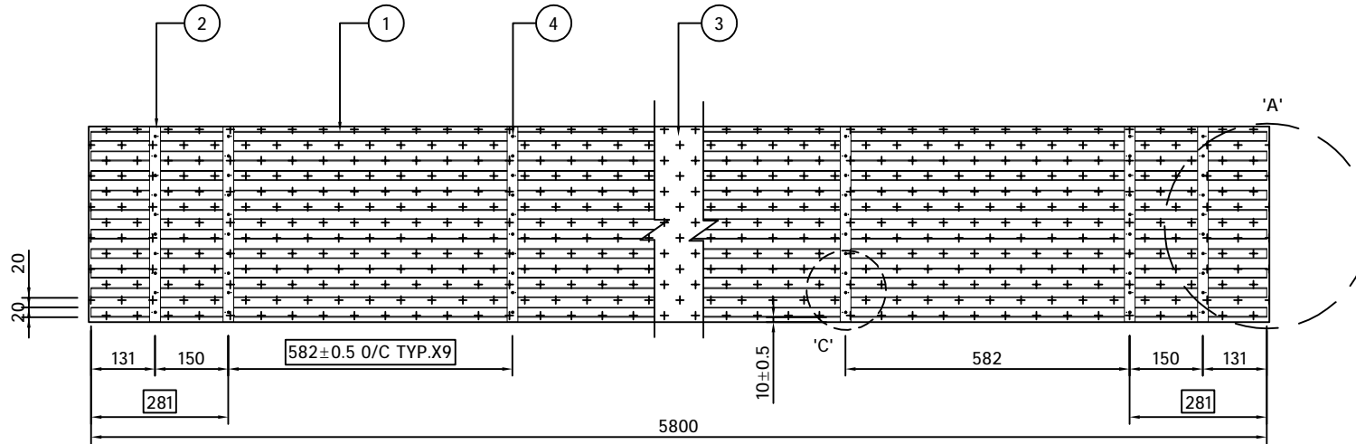
TOP VIEW SCALE:1:4
