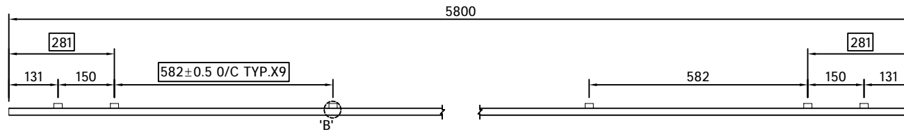
FRONT VIEW SCALE:1:4
