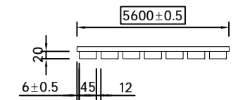
SIDE VIEW SCALE 1:14
