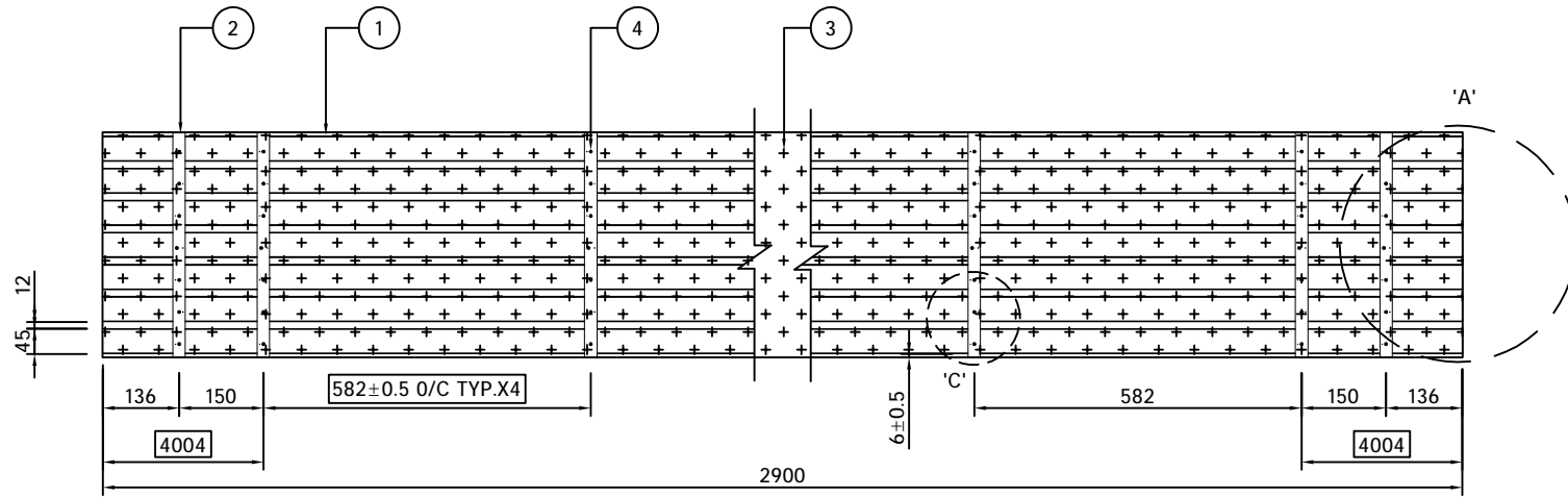
TOP VIEW SCALE 1:14
